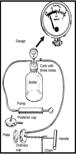
Figure E4. 4 A vacuum extraction system showing the pressure gauge
